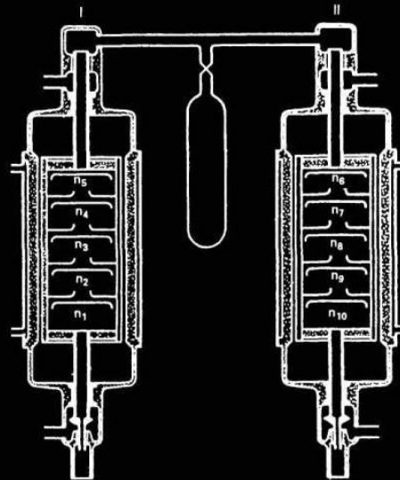
Harteck's double rocking gas centrifuges
