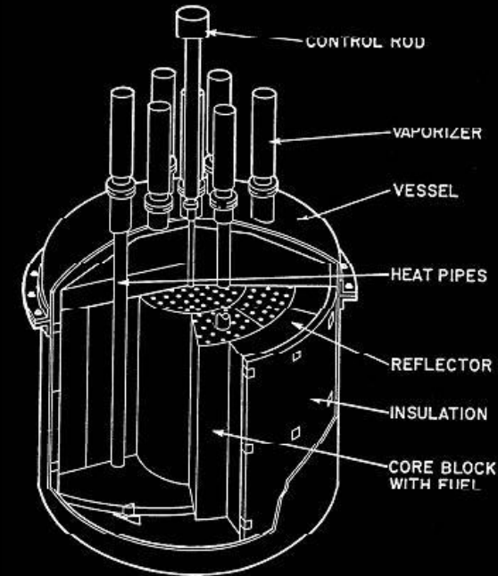
AECL Nuclear Battery proposal; 1988
